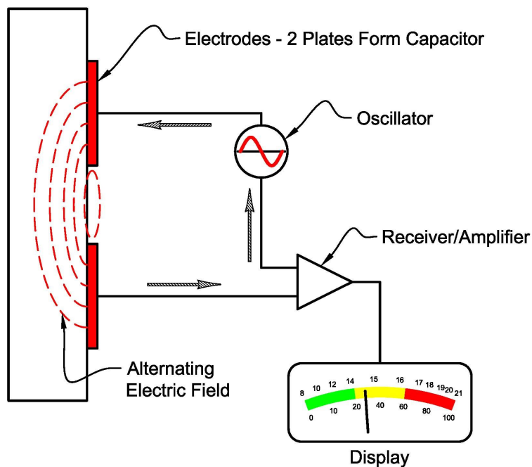
Moisture Meter Circuit
